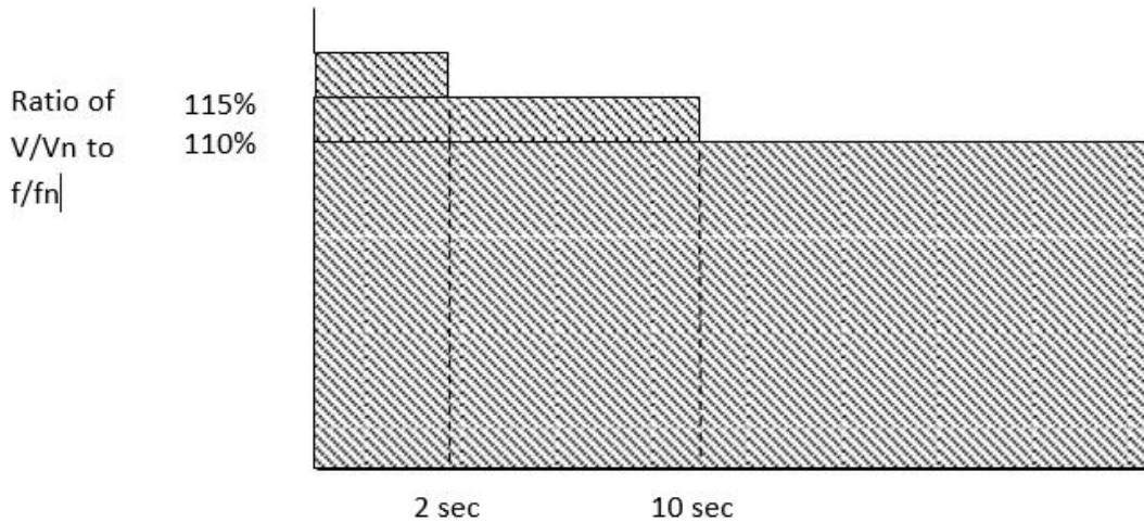
Figure 5: Response to Voltage – Frequency disturbances
