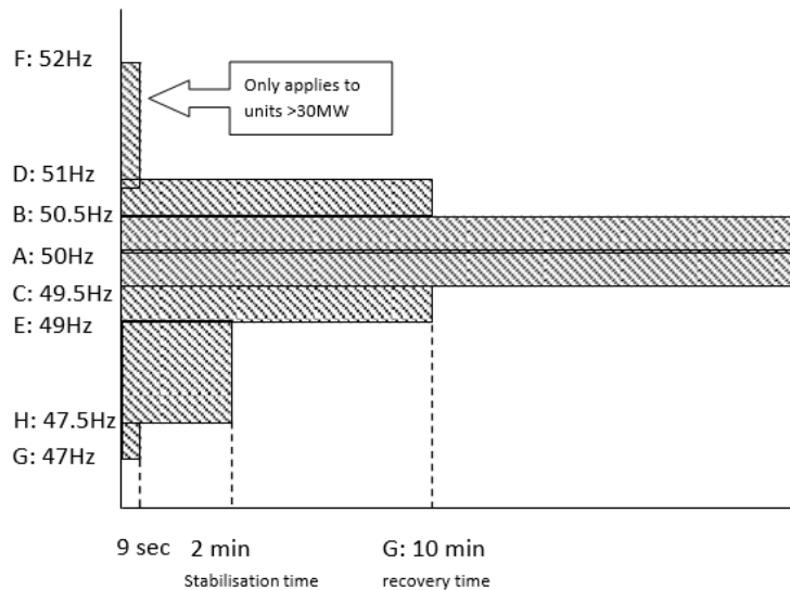
Figure 3: Frequency disturbance response minimum access standard
