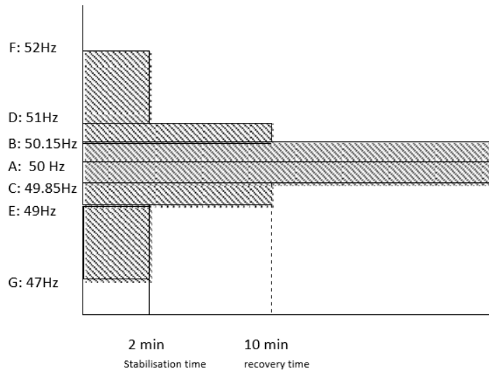
Figure 2: Frequency disturbance response automatic access standard
