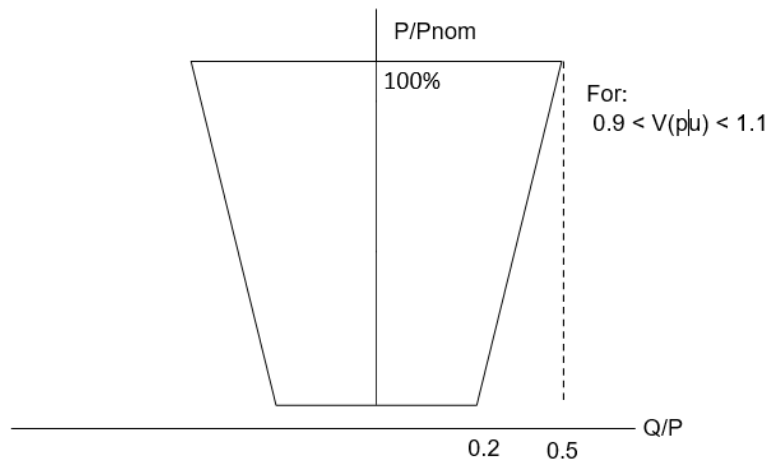
Figure 1: Reactive power capability diagram (example only) – note that this is an example of a negotiated standard as it is not capable of Q = 0.395 \times P for all levels of active power.
