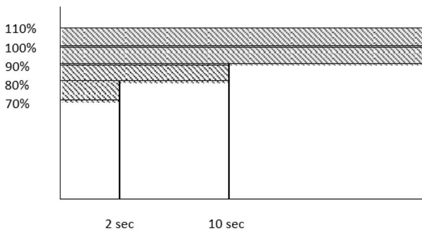
Figure 5: Response to voltage disturbances under 110 per cent
