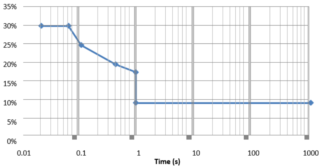
Figure 4: Response to voltage disturbances over 110 per cent, automatic access standard
