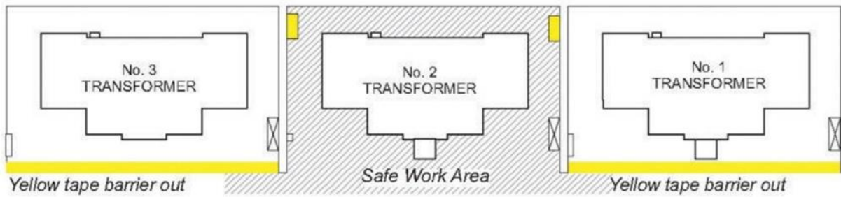
Figure 6. Examples and diagram illustrating correct entry to a safe work area barrier out.
