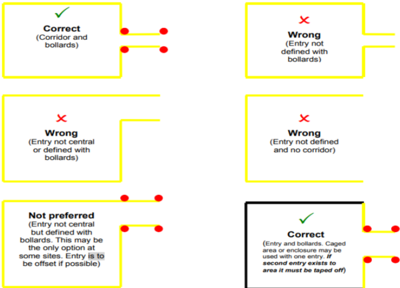
Figure 3. Entries to Access Authority areas in outdoor switchyards
